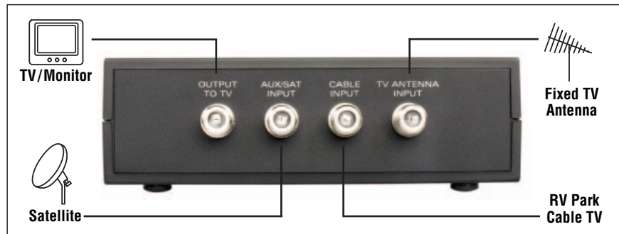
Rear Panel Connections
